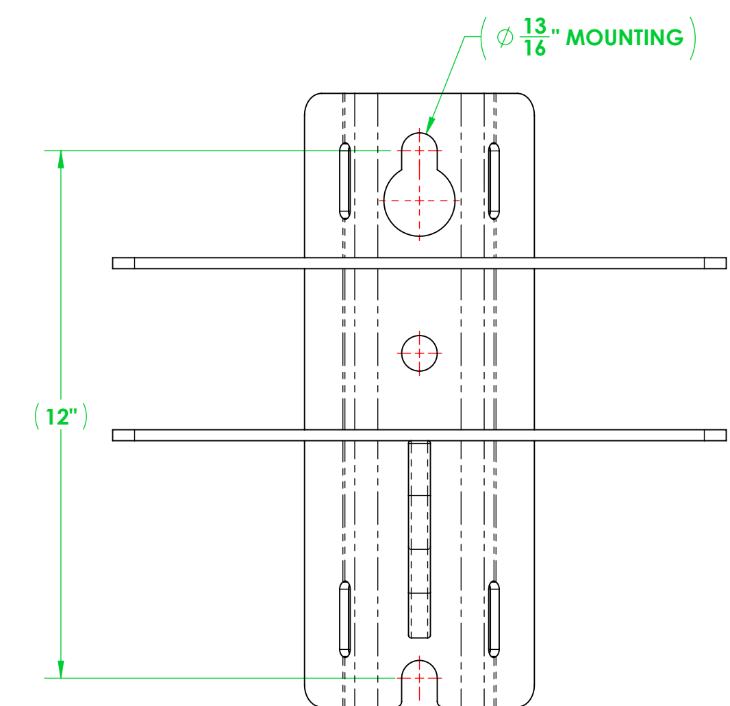
DETAIL A
